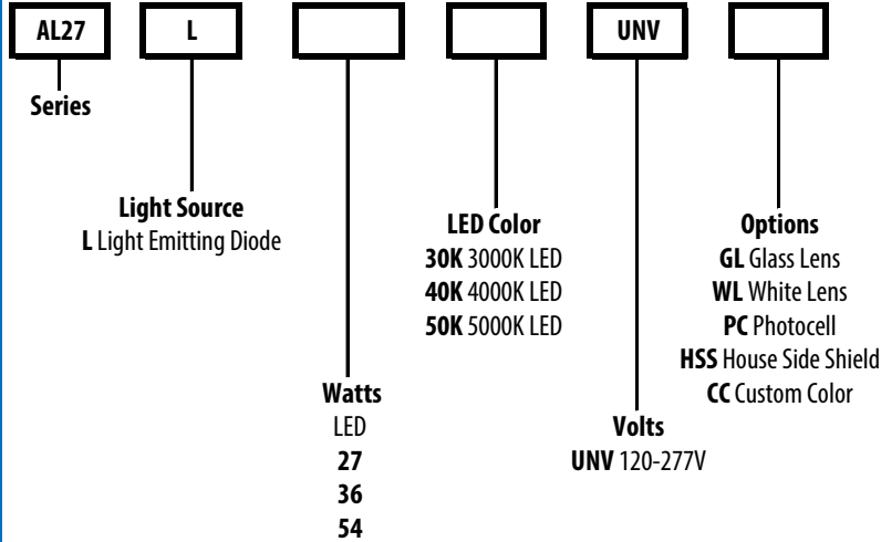
AL27 LED Series
