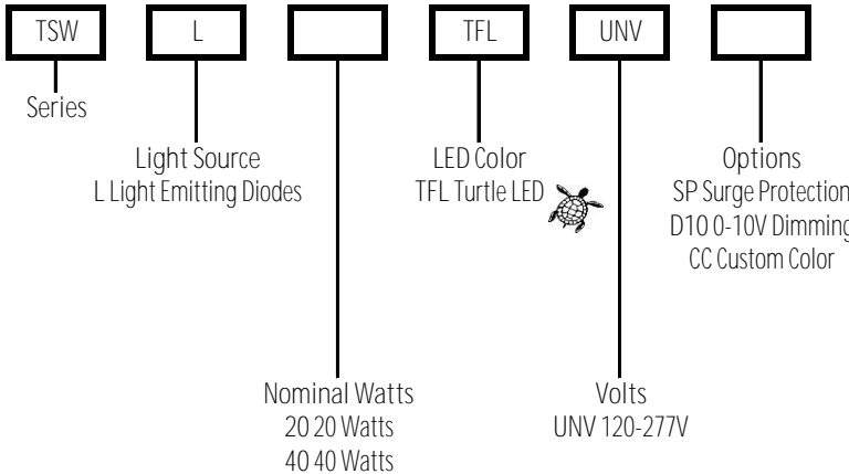
TSW Amber LED Series
