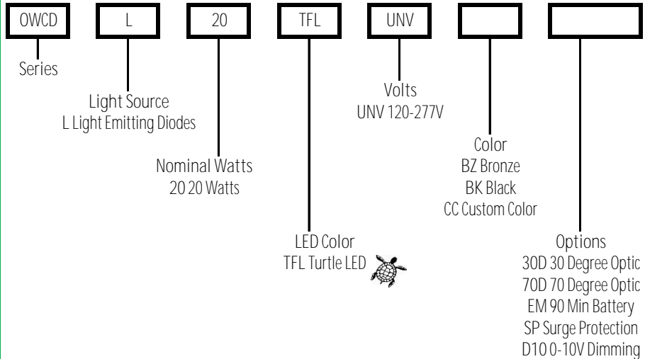
OWCD Amber LED Series
