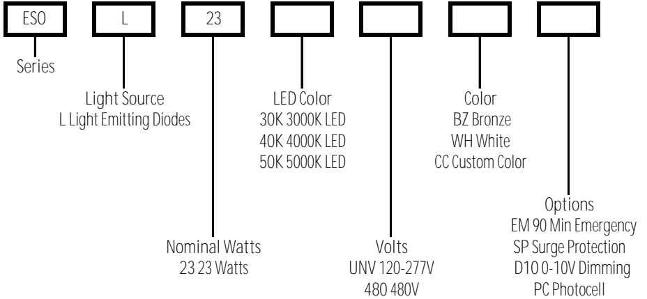
ESO LED Series
