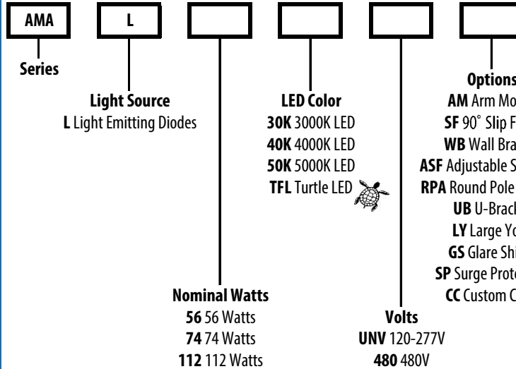
AMA LED Series
