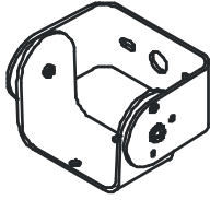
UBS Small 2 Piece Swivel U-Bracket Designed to hold fixtures up to 400 Watt HID; uses standard hole patterns to mount to fixture; Bronze Steel
