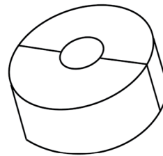
PBC-RR* Pole Base Cover Round-Round 2 Piece Aluminum Construction for 3, 4, 4.5, 5 and 6" Round Poles. Specify Pole Size, Desired Width, and Depth. Standard Bronze, Optional Colors.
